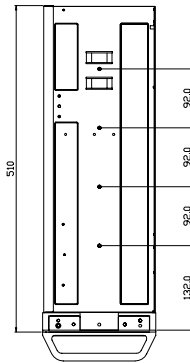
Right-side View
